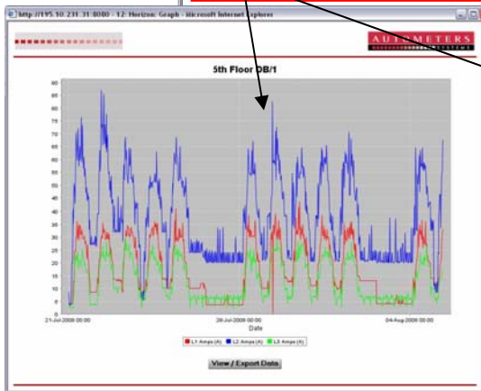
3 Phase Current Load
